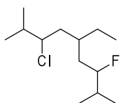
3-chloro-5-ethyl-7-fluoro-2,8-dimethylnonane
