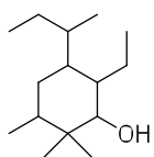
5-(sec-butyl)-6-ethyl-2,2,3-trimethylcyclohexan-1-ol
