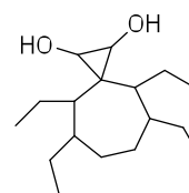
4,5,8,9-tetraethylspiro[2.6]nonane-1,2-diol
