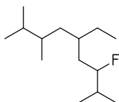
5-ethyl-3-fluoro-2,7,8-trimethylnonane
