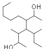
4-(sec-butyl)-3-methyl-5-pentylheptane-2,6-diol
