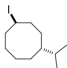
trans -1-iodo-4-isopropylcyclooctane
