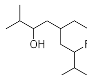
5-ethyl-7-fluoro-2,8-dimethylnonane-3-ol
