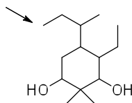
5-(sec-butyl)-4-ethyl-2,2-dimethylcyclohexane-1,3-diol
