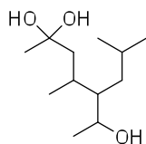
5-isobutyl-4-methylheptane-2,2,6-triol
